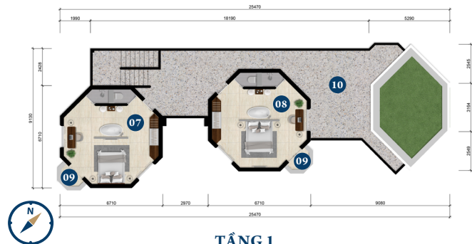
TẦNG 1 1st FLOOR
