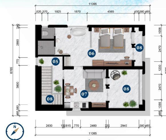
TẦNG 1 1st FLOOR
