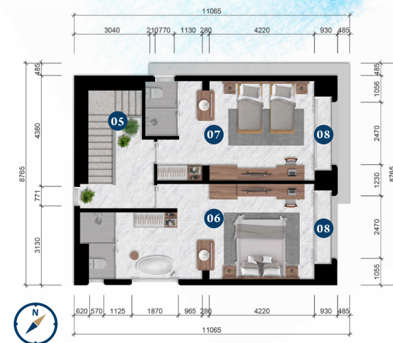
TẦNG 1 1st FLOOR
